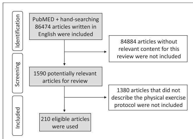
Fig. 1. - Flowchart of literature search.
